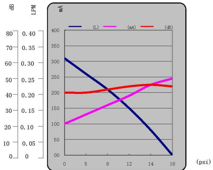
Characteristic Curve
