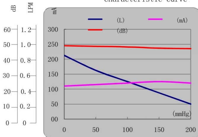
Characteristic Curve.
