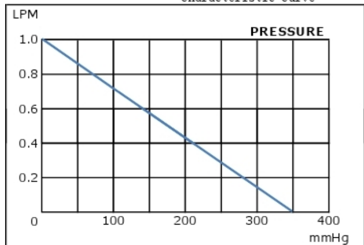
Characteristic Curve
