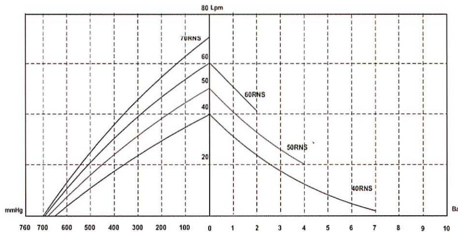
Rocking Piston Pump (Single Head)
