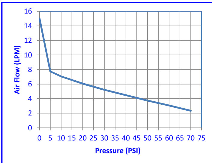
Pressure Output Air Flow
