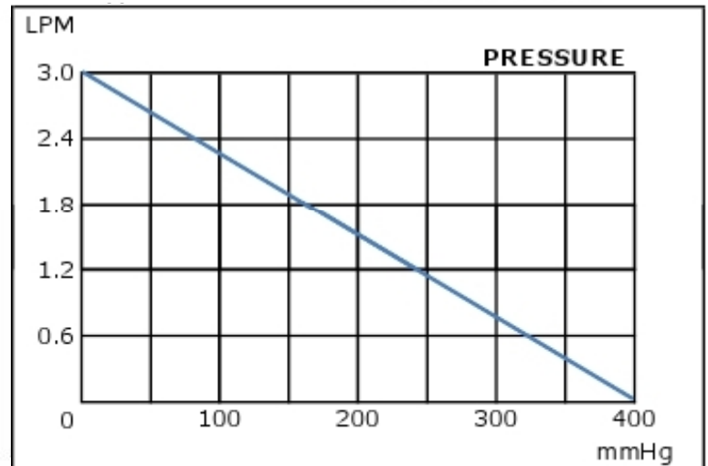
Characteristic Curve
