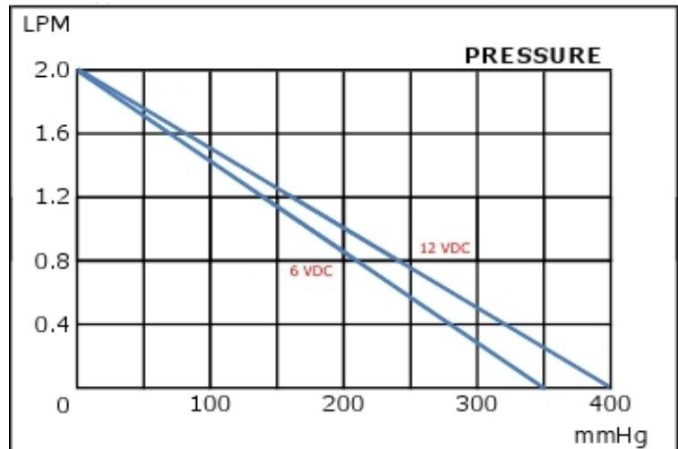
Characteristic Curve
