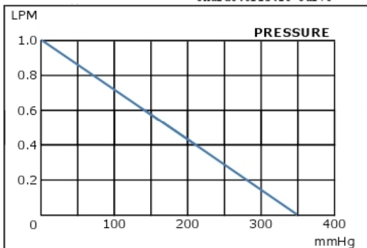
Characteristic Curve
