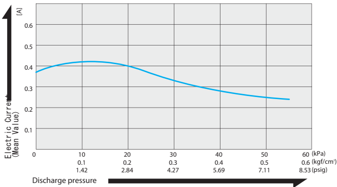
Current Characteristics
