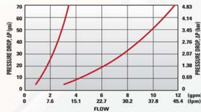
40CB Series Water Flow
