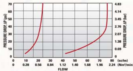
40CB Series Air Flow
